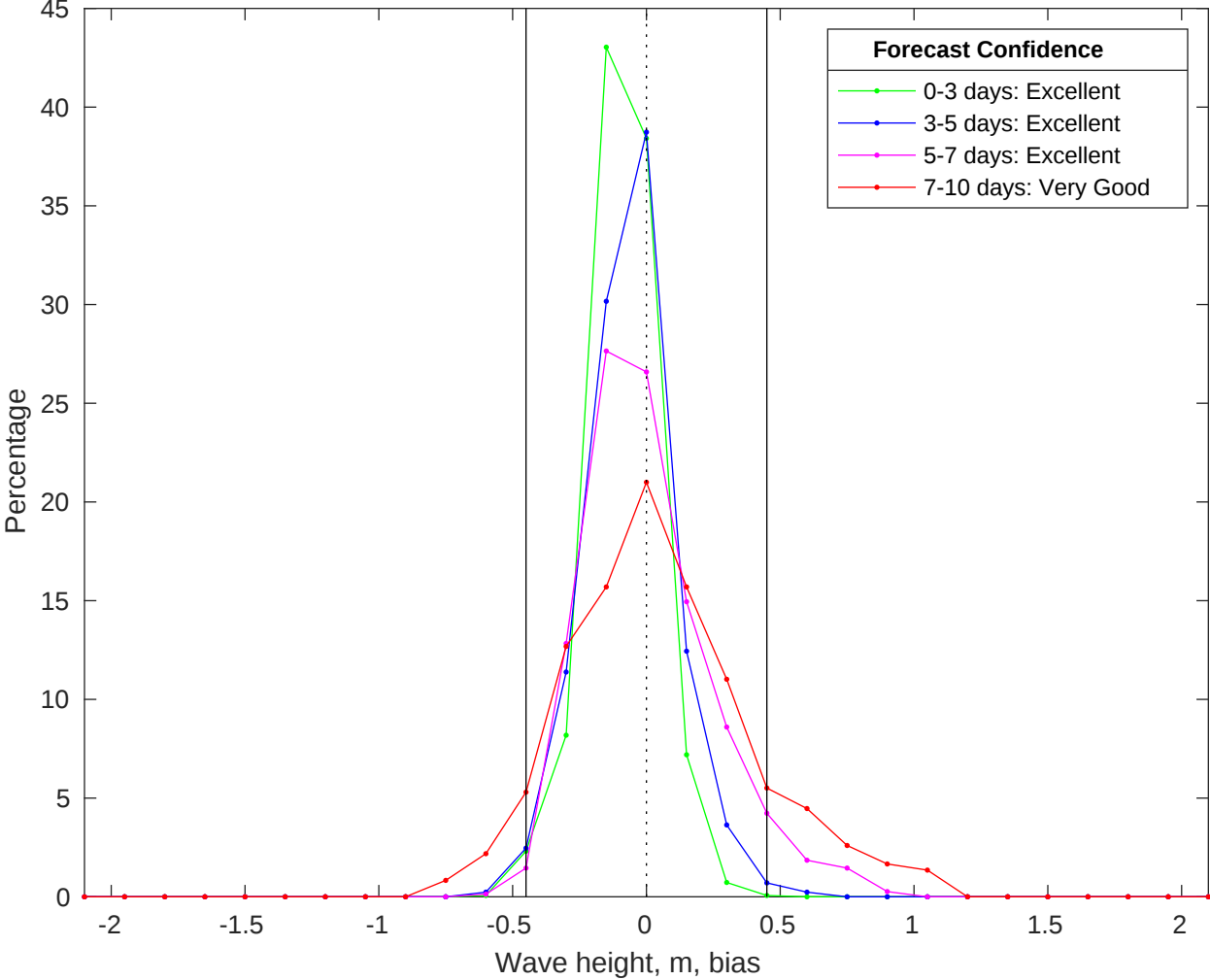
NDBC 42019 vs CMEMS Waves Bias Histogram: 12-Jun-2025
