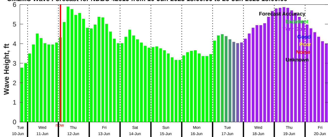
CMEMS Wave Forecast for NDBC 42019 from 10-Jun-2025 18:00:00 to 20-Jun-2025 18:00:00
