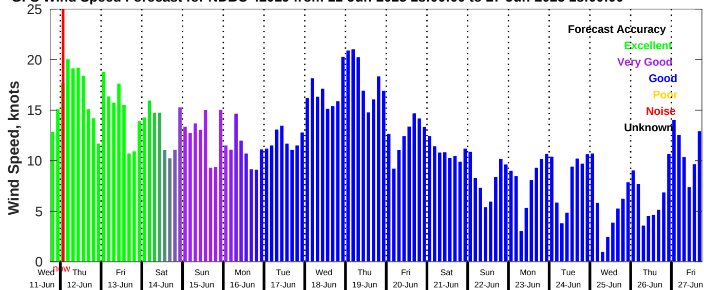
GFS Wind Speed Forecast for NDBC 42019 from 11-Jun-2025 18:00:00 to 27-Jun-2025 18:00:00
