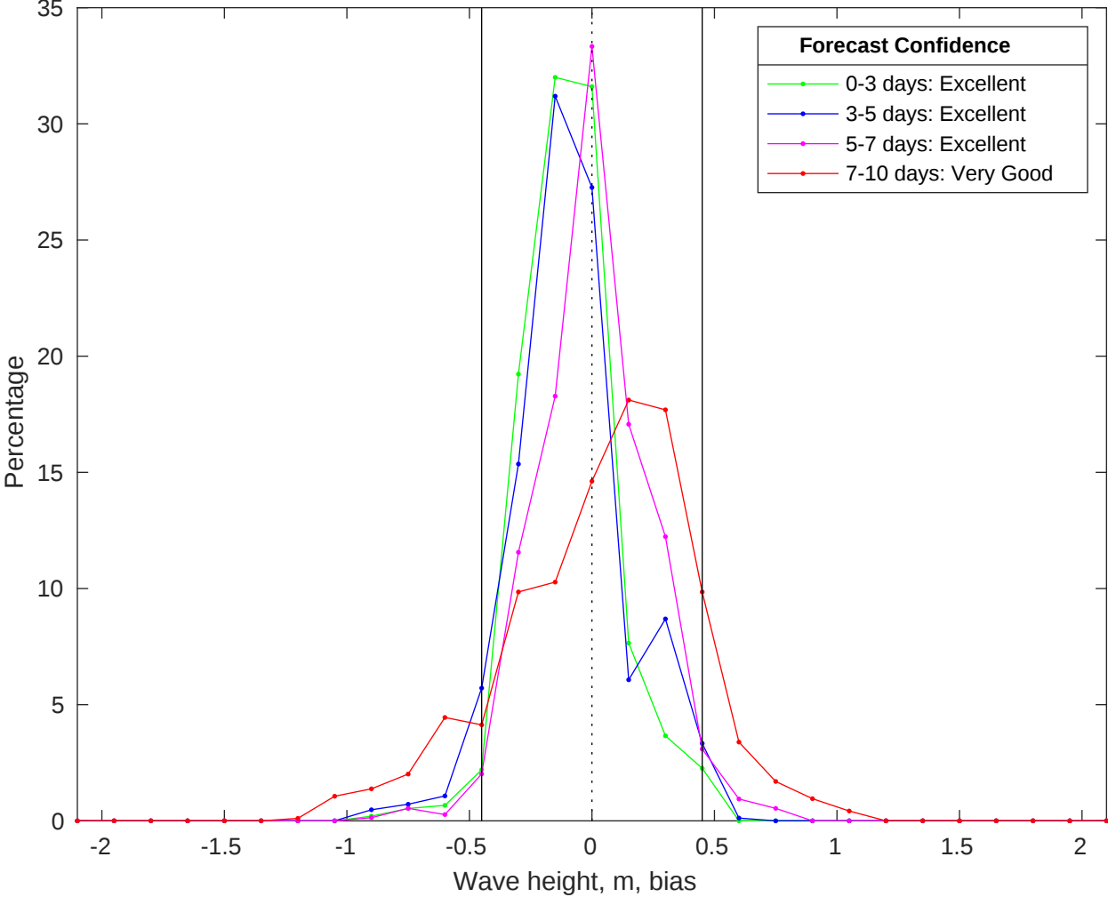
NDBC 42020 vs CMEMS Waves Bias Histogram: 12-Jun-2025
