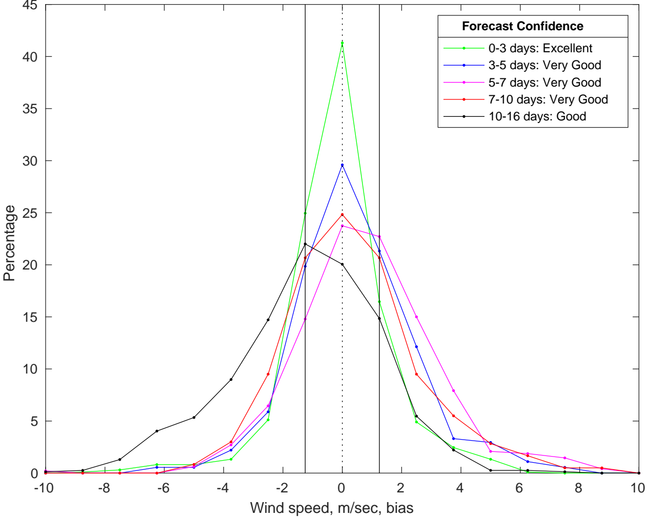
NDBC 42020 vs GFS Winds Bias Histogram: 12-Jun-2025
