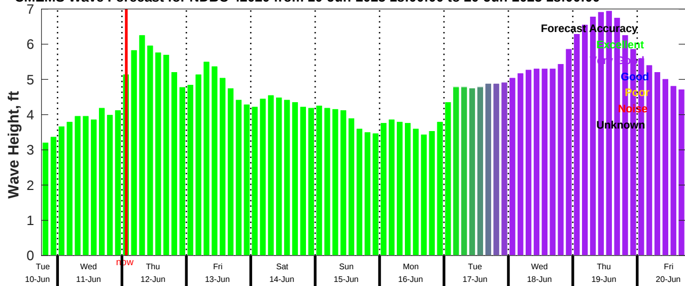
CMEMS Wave Forecast for NDBC 42020 from 10-Jun-2025 18:00:00 to 20-Jun-2025 18:00:00
