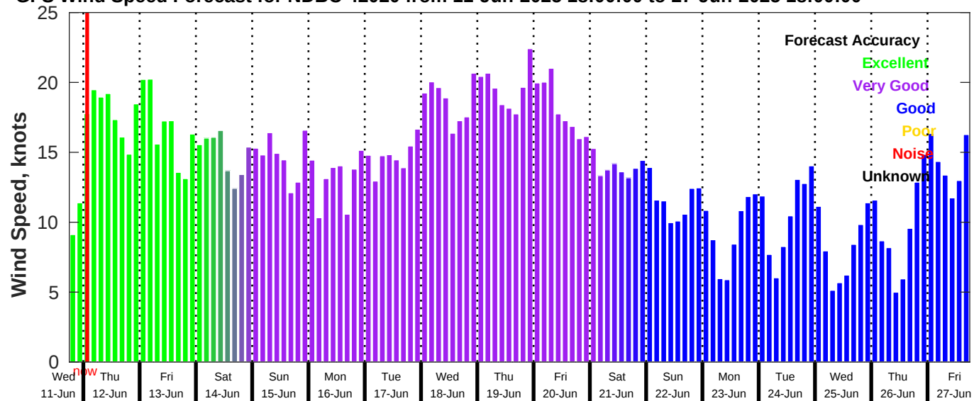
GFS Wind Speed Forecast for NDBC 42020 from 11-Jun-2025 18:00:00 to 27-Jun-2025 18:00:00
