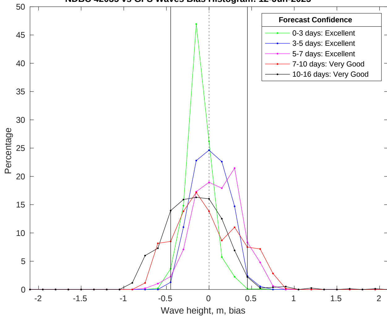
NDBC 42035 vs GFS Waves Bias Histogram: 12-Jun-2025
