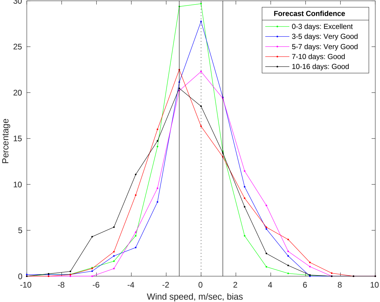
NDBC 42035 vs GFS Winds Bias Histogram: 12-Jun-2025
