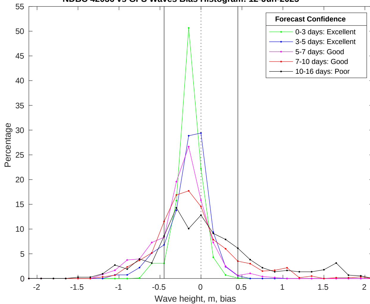
NDBC 42036 vs GFS Waves Bias Histogram: 12-Jun-2025
