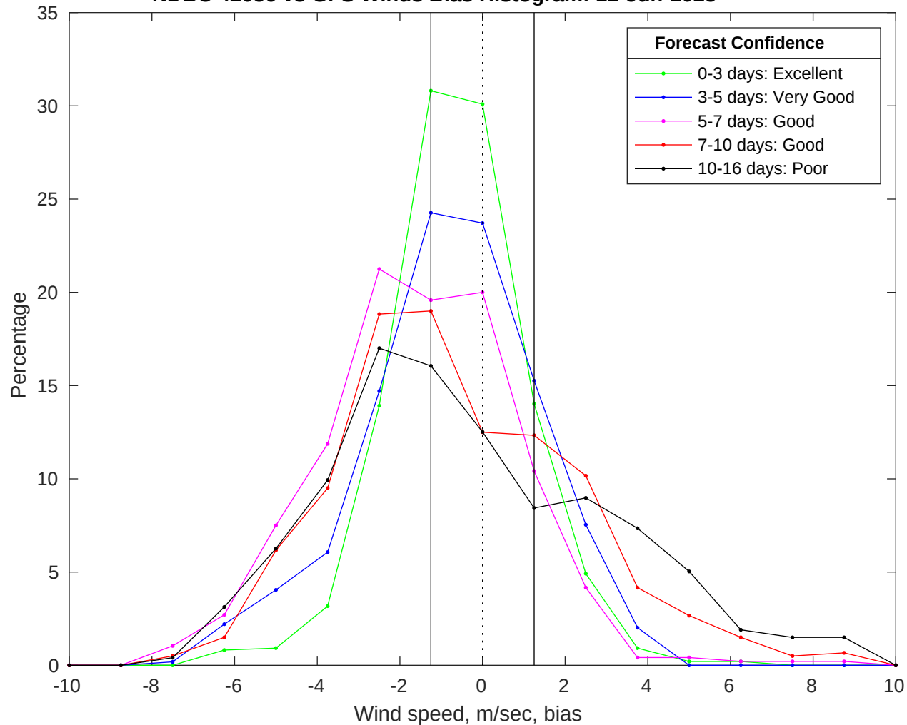
NDBC 42036 vs GFS Winds Bias Histogram: 12-Jun-2025
