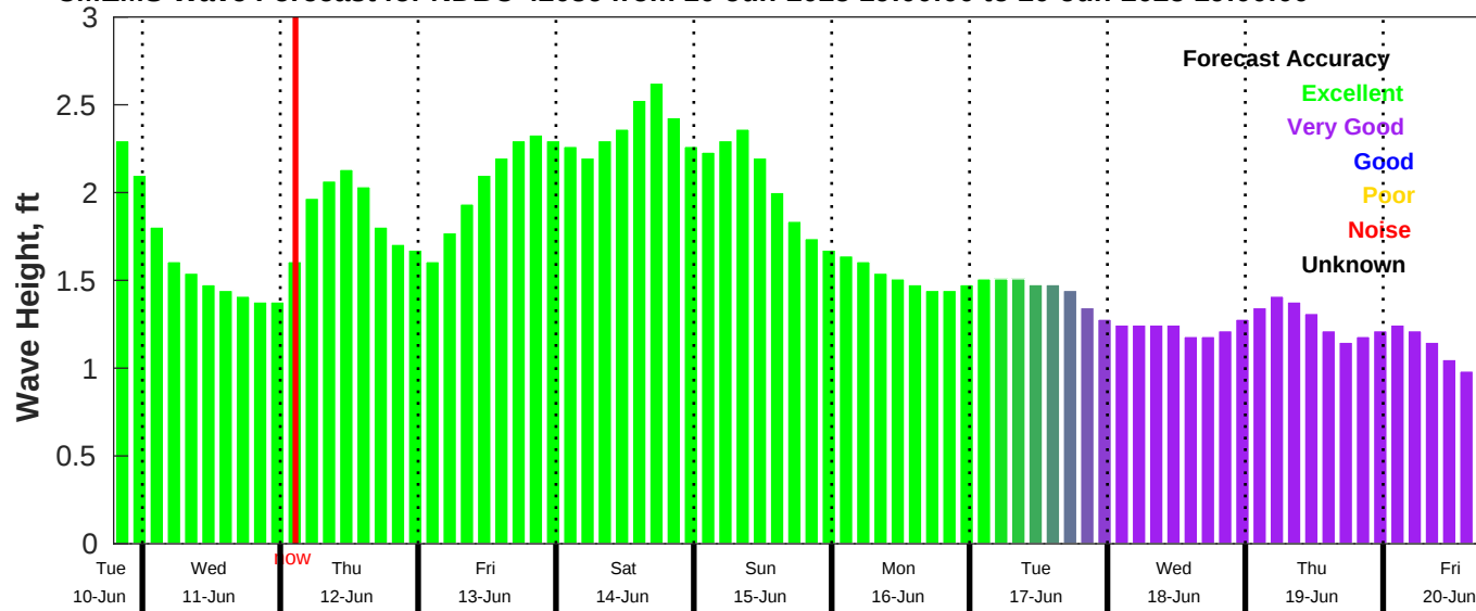
CMEMS Wave Forecast for NDBC 42036 from 10-Jun-2025 19:00:00 to 20-Jun-2025 19:00:00
