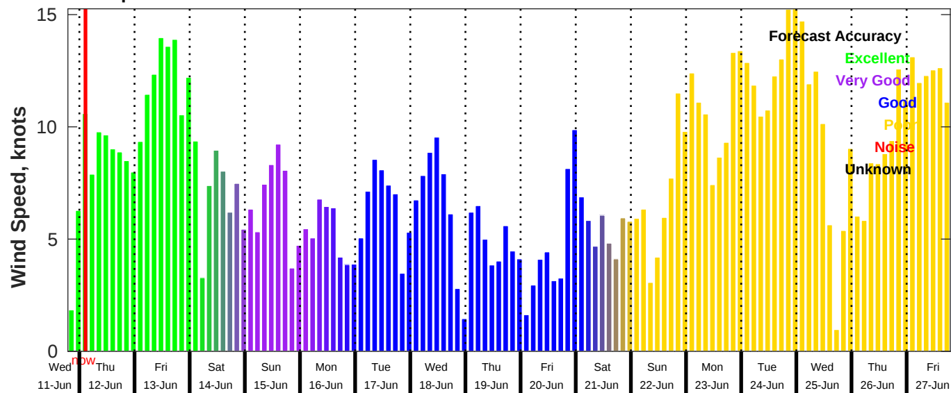
GFS Wind Speed Forecast for NDBC 42036 from 11-Jun-2025 19:00:00 to 27-Jun-2025 19:00:00
