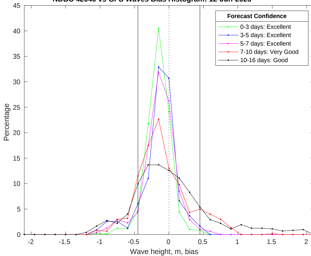
NDBC 42040 vs GFS Waves Bias Histogram: 12-Jun-2025
