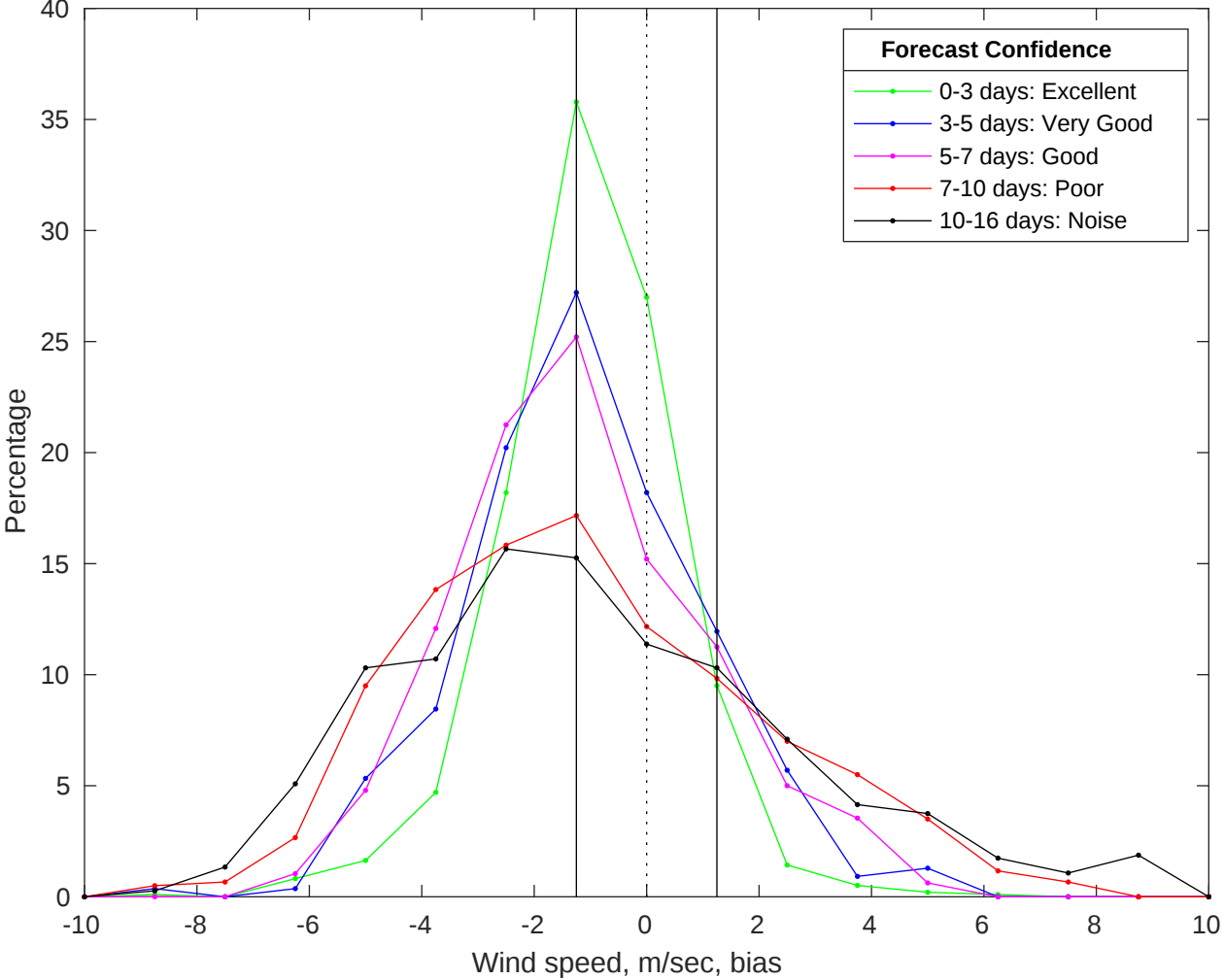
NDBC 42040 vs GFS Winds Bias Histogram: 12-Jun-2025
