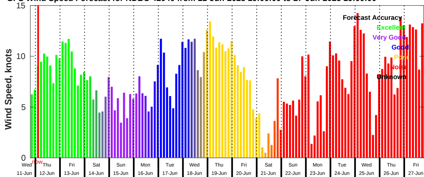
GFS Wind Speed Forecast for NDBC 42040 from 11-Jun-2025 19:00:00 to 27-Jun-2025 19:00:00
