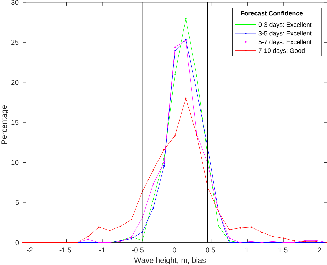
NDBC 46011 vs CMEMS Waves Bias Histogram: 12-Jun-2025
