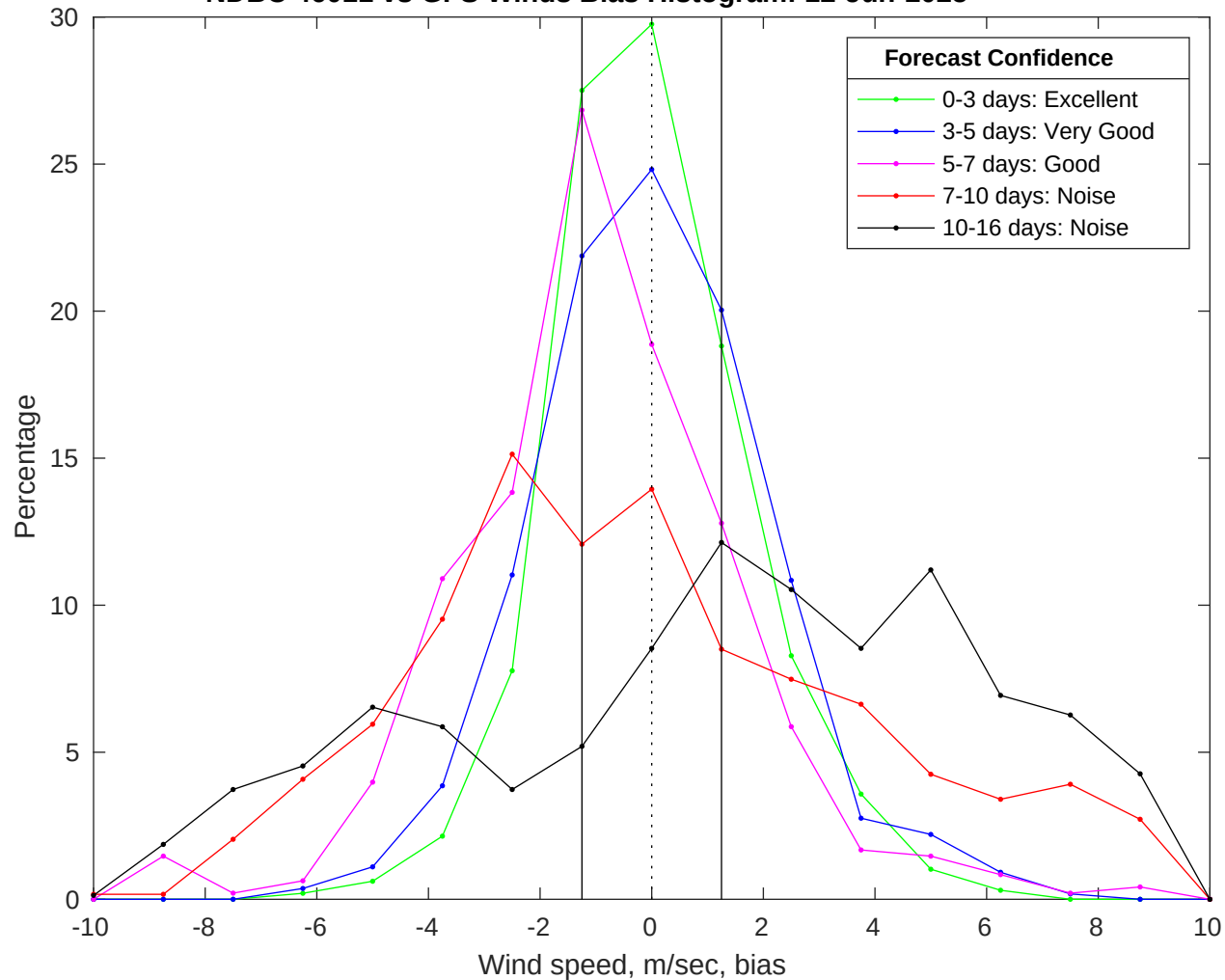
NDBC 46011 vs GFS Winds Bias Histogram: 12-Jun-2025
