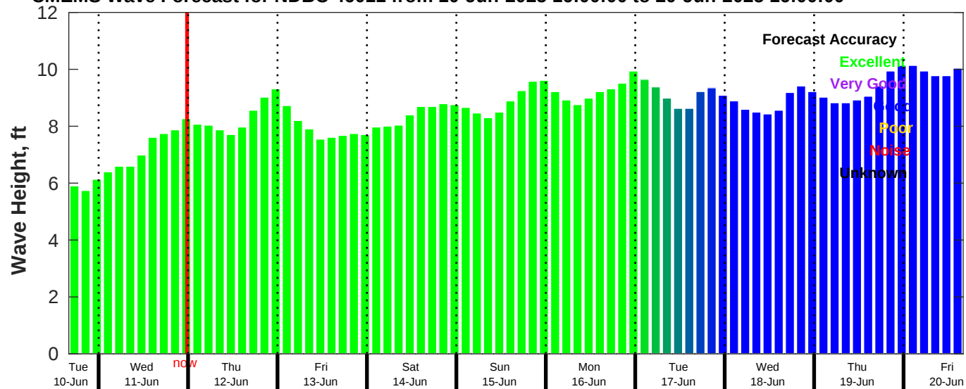
CMEMS Wave Forecast for NDBC 46011 from 10-Jun-2025 16:00:00 to 20-Jun-2025 16:00:00
