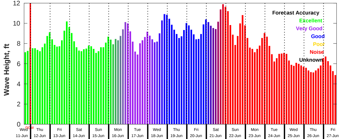
GFS Wave Forecast for NDBC 46011 from 11-Jun-2025 16:00:00 to 27-Jun-2025 16:00:00
