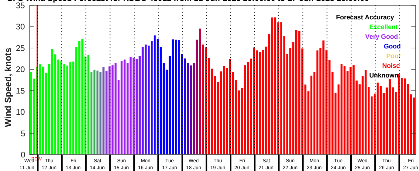
GFS Wind Speed Forecast for NDBC 46011 from 11-Jun-2025 16:00:00 to 27-Jun-2025 16:00:00
