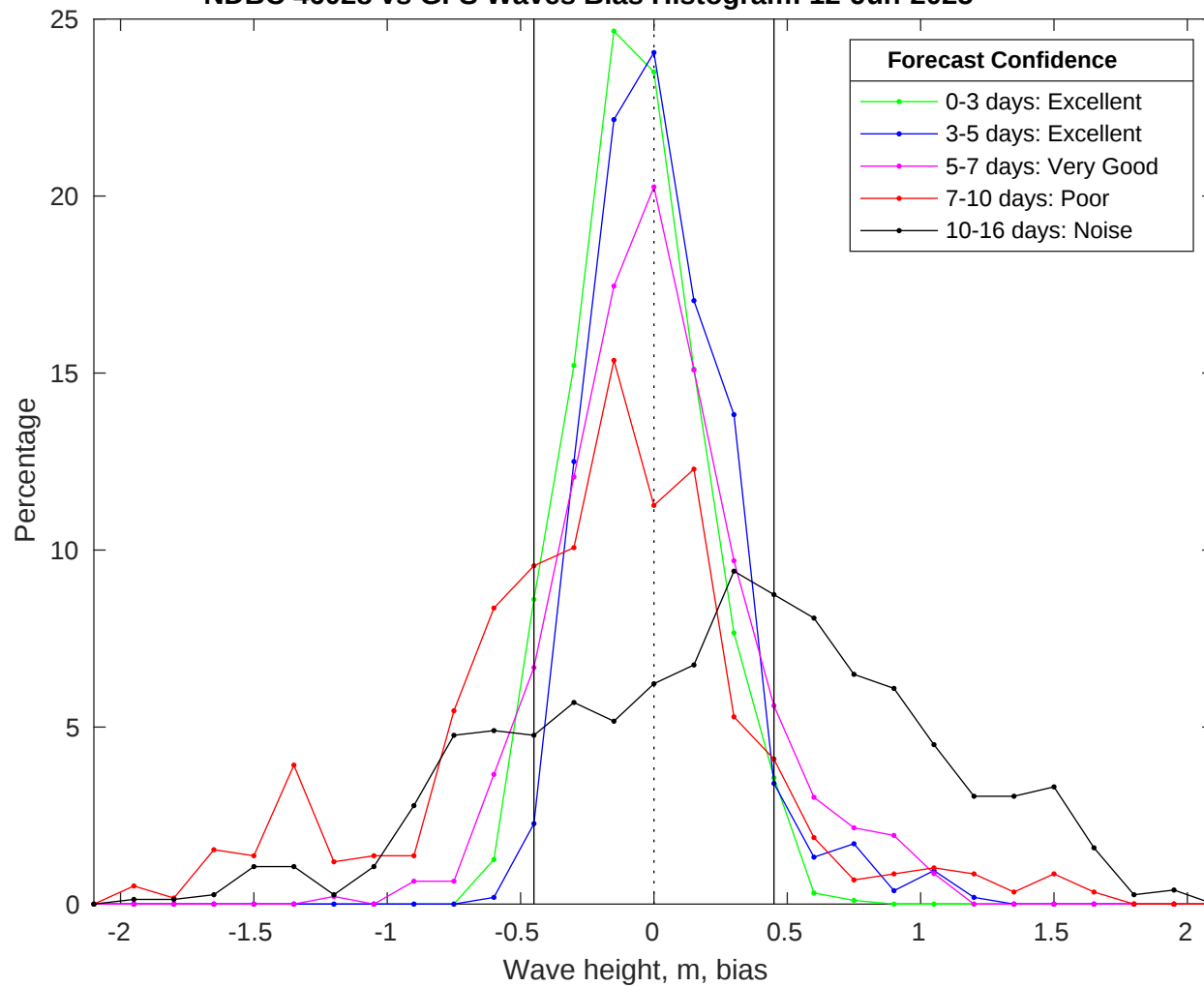
NDBC 46028 vs GFS Waves Bias Histogram: 12-Jun-2025
