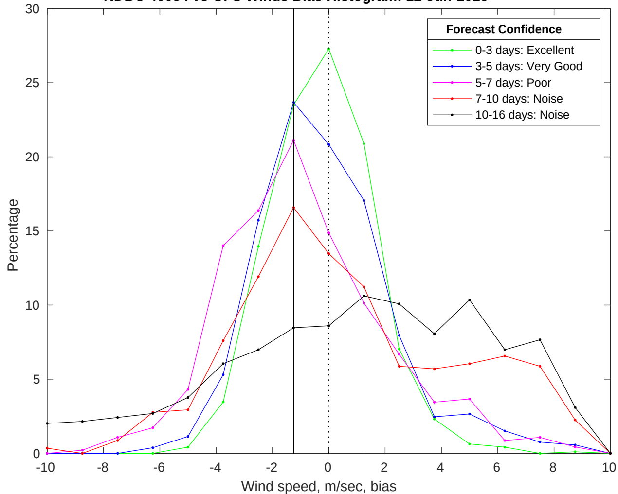
NDBC 46054 vs GFS Winds Bias Histogram: 12-Jun-2025
