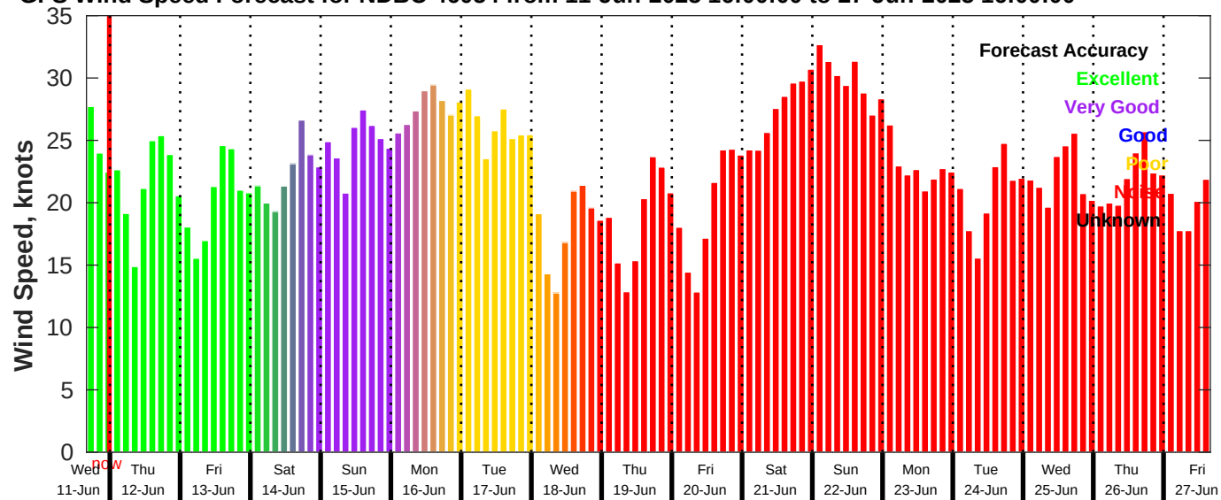
GFS Wind Speed Forecast for NDBC 46054 from 11-Jun-2025 16:00:00 to 27-Jun-2025 16:00:00
