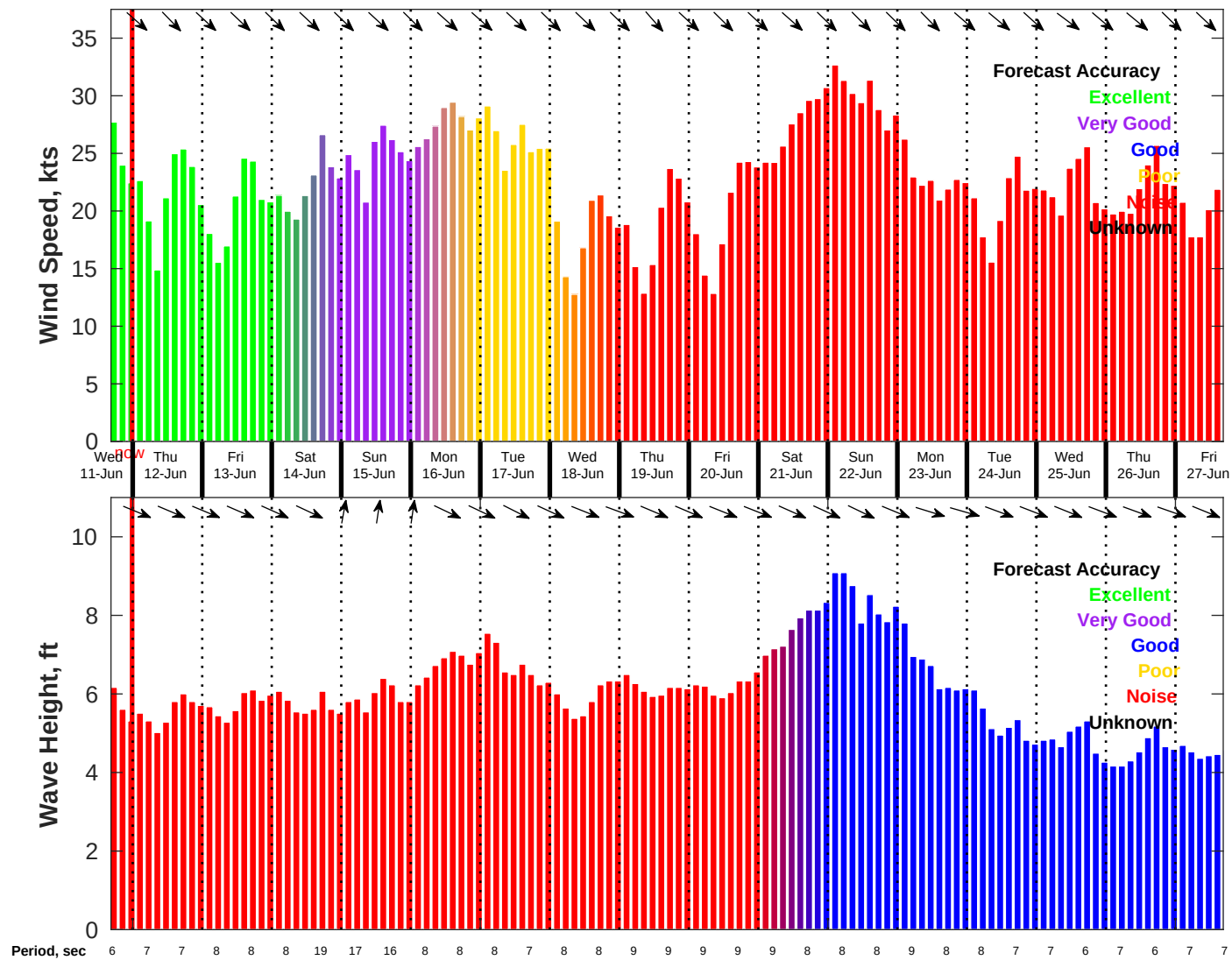
Wind & Wave Forecast for NDBC 46054 from 11-Jun-2025 16:00:00 to 27-Jun-2025 16:00:00
