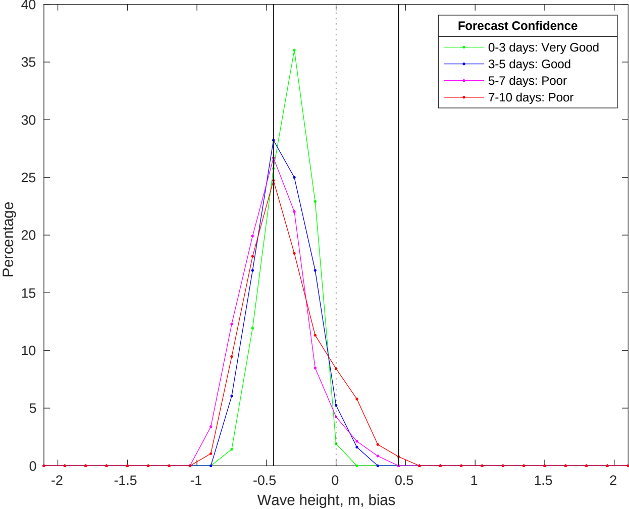
NDBC 51209 vs CMEMS Waves Bias Histogram: 12-Jun-2025
