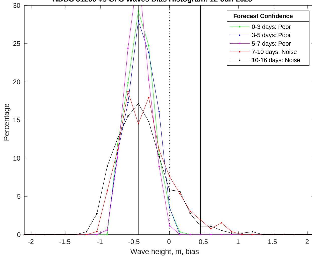
NDBC 51209 vs GFS Waves Bias Histogram: 12-Jun-2025
