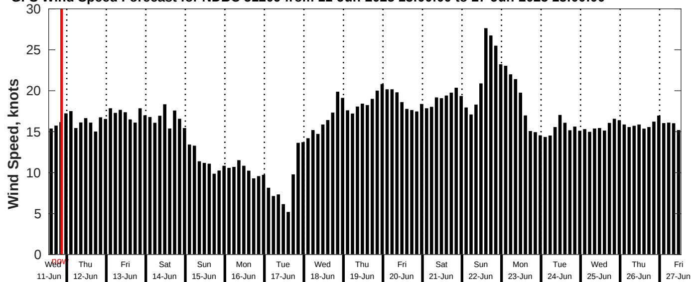
GFS Wind Speed Forecast for NDBC 51209 from 11-Jun-2025 13:00:00 to 27-Jun-2025 13:00:00
