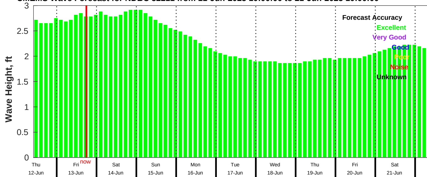
CMEMS Wave Forecast for NDBC 52211 from 11-Jun-2025 10:00:00 to 21-Jun-2025 10:00:00
