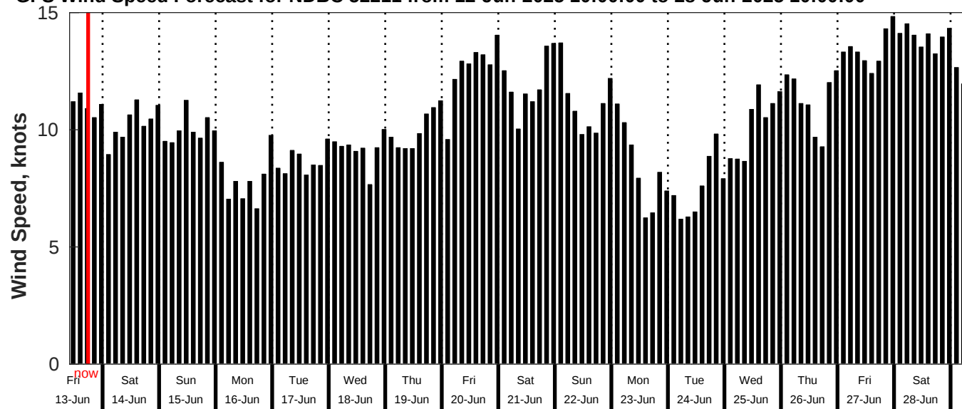
GFS Wind Speed Forecast for NDBC 52211 from 12-Jun-2025 10:00:00 to 28-Jun-2025 10:00:00
