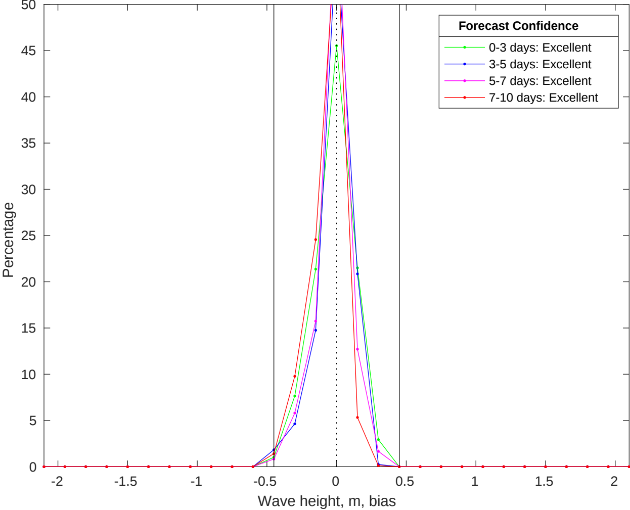
NDBC 52212 vs CMEMS Waves Bias Histogram: 12-Jun-2025
