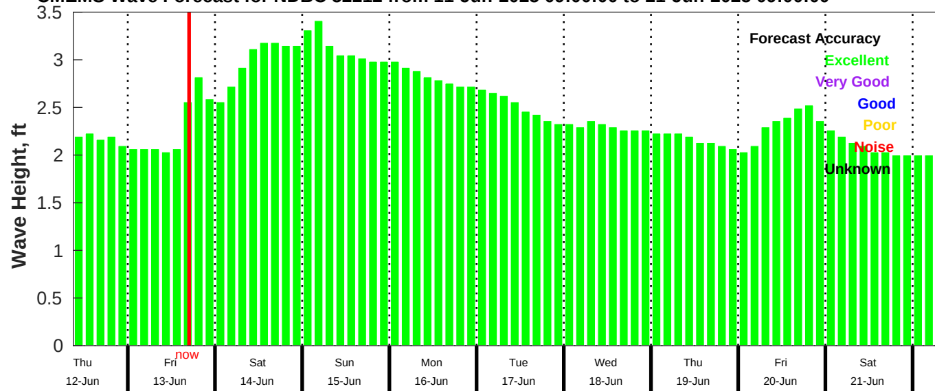
CMEMS Wave Forecast for NDBC 52212 from 11-Jun-2025 09:00:00 to 21-Jun-2025 09:00:00
