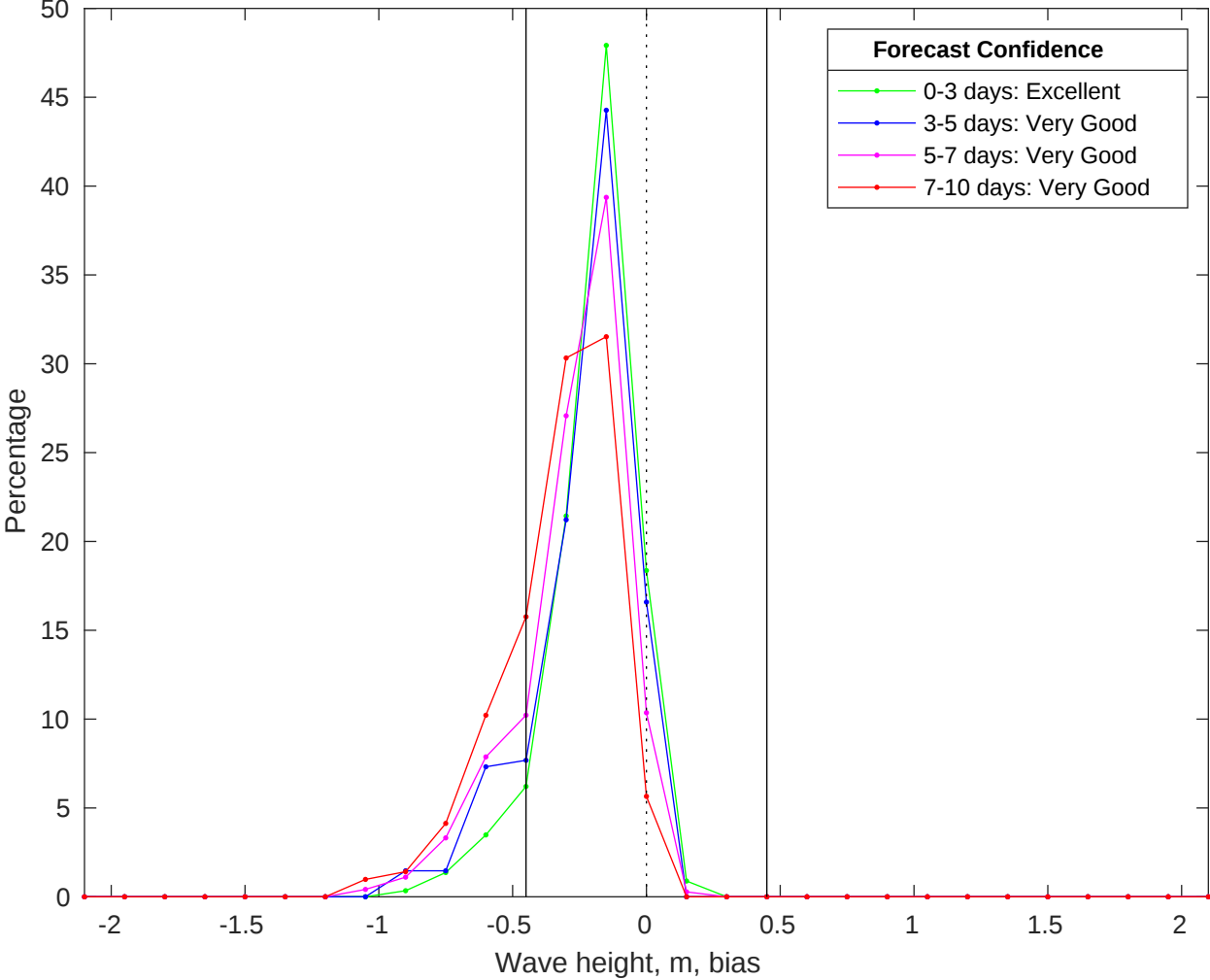
NDBC 52213 vs CMEMS Waves Bias Histogram: 12-Jun-2025
