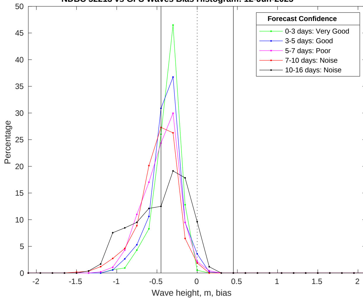
NDBC 52213 vs GFS Waves Bias Histogram: 12-Jun-2025
