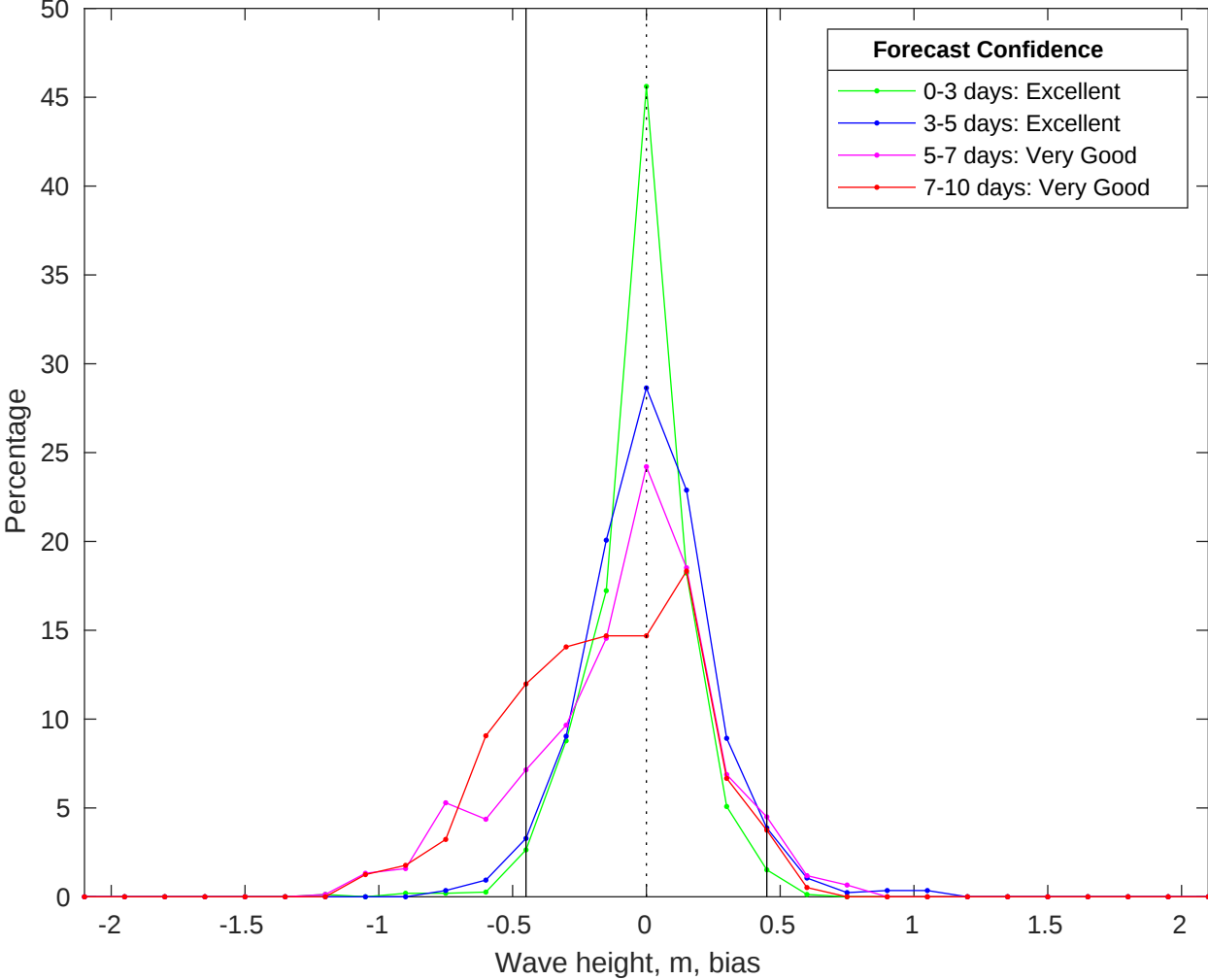
NDBC 41004 vs CMEMS Waves Bias Histogram: 13-Jun-2025
