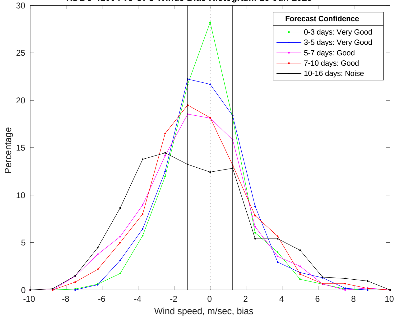
NDBC 41004 vs GFS Winds Bias Histogram: 13-Jun-2025
