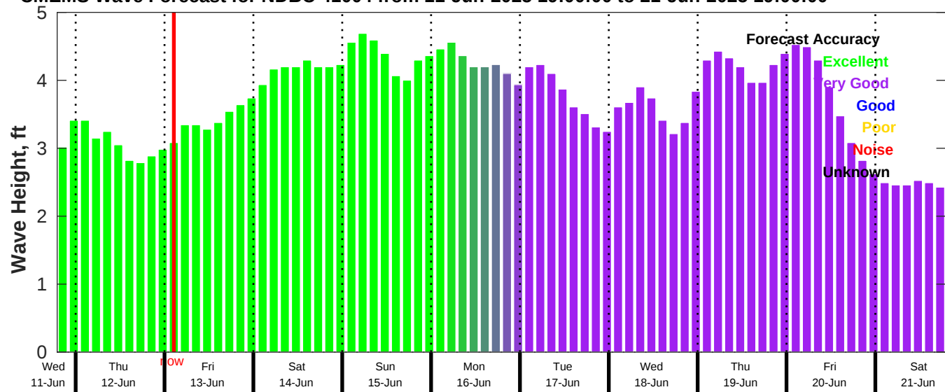
CMEMS Wave Forecast for NDBC 41004 from 11-Jun-2025 19:00:00 to 21-Jun-2025 19:00:00
