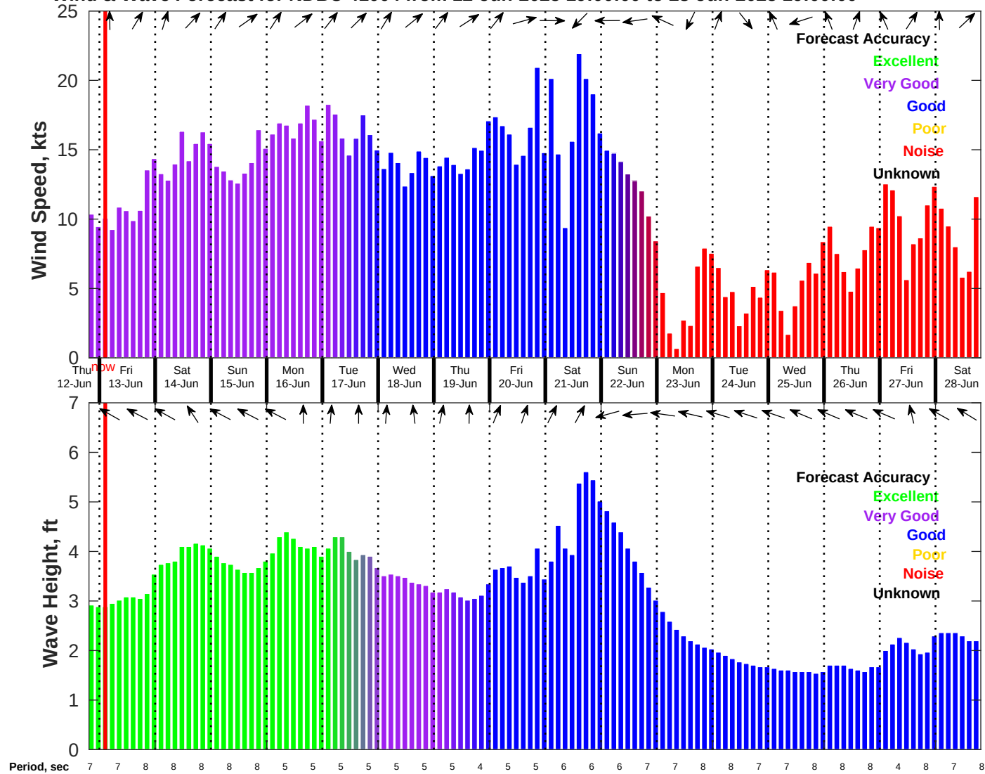
Wind & Wave Forecast for NDBC 41004 from 12-Jun-2025 19:00:00 to 28-Jun-2025 19:00:00
