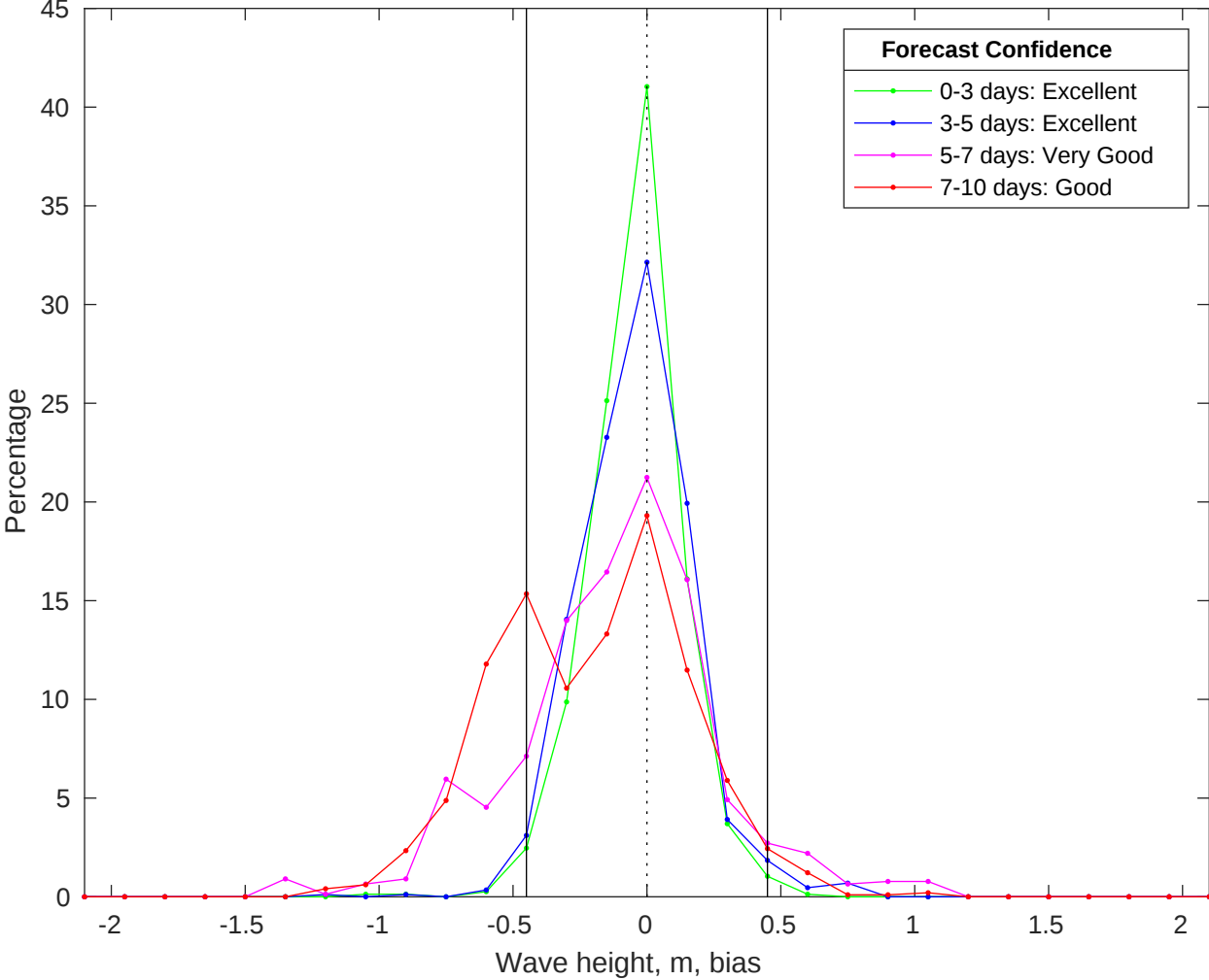
NDBC 41013 vs CMEMS Waves Bias Histogram: 13-Jun-2025
