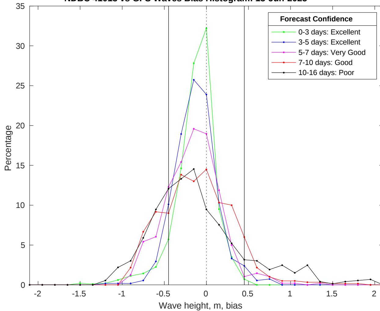
NDBC 41013 vs GFS Waves Bias Histogram: 13-Jun-2025
