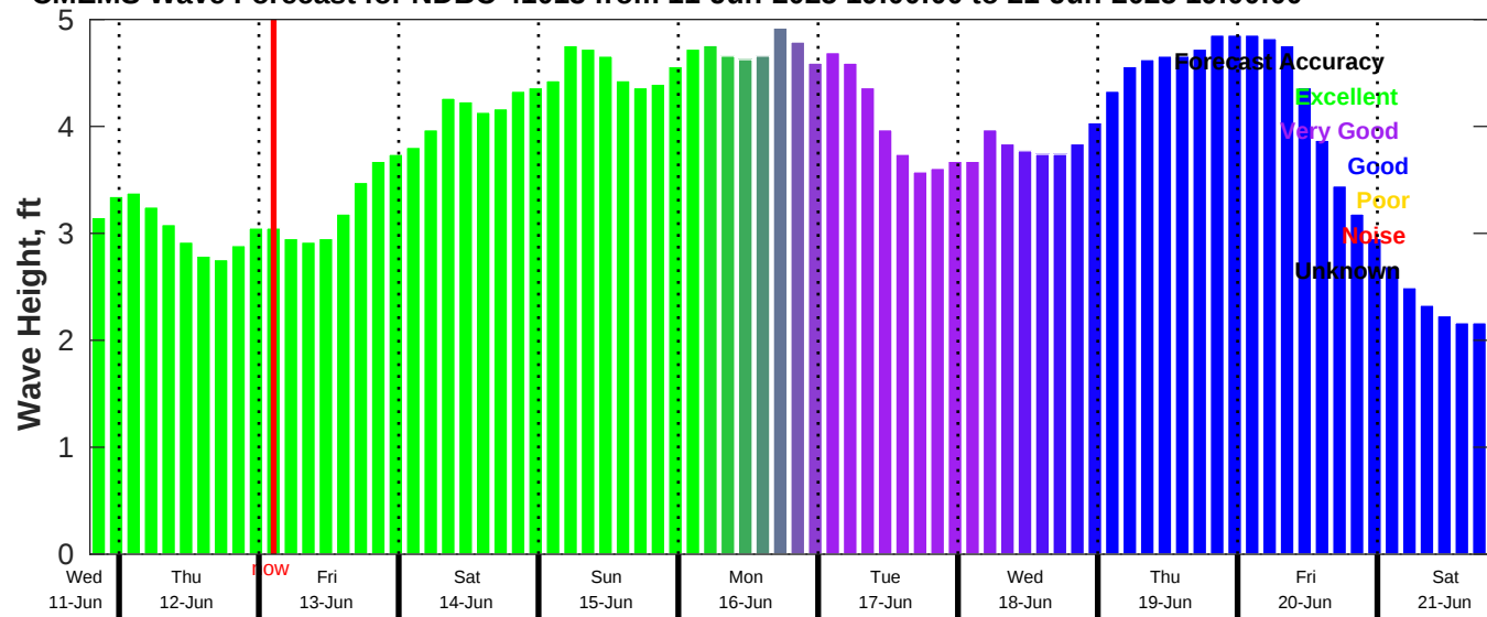
CMEMS Wave Forecast for NDBC 41013 from 11-Jun-2025 19:00:00 to 21-Jun-2025 19:00:00
