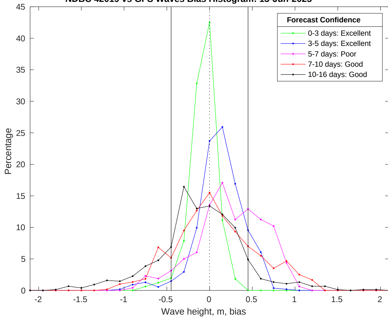
NDBC 42019 vs GFS Waves Bias Histogram: 13-Jun-2025
