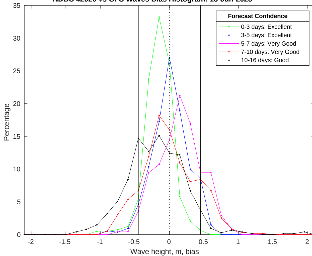
NDBC 42020 vs GFS Waves Bias Histogram: 13-Jun-2025
