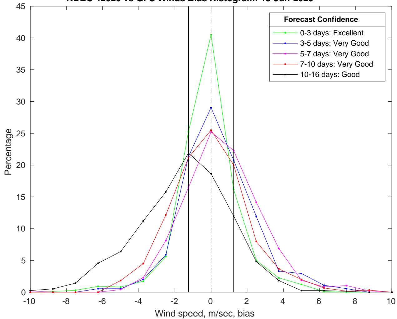
NDBC 42020 vs GFS Winds Bias Histogram: 13-Jun-2025
