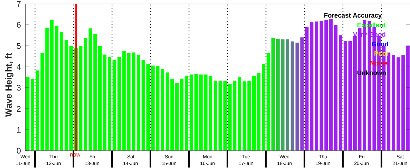
CMEMS Wave Forecast for NDBC 42020 from 11-Jun-2025 18:00:00 to 21-Jun-2025 18:00:00
