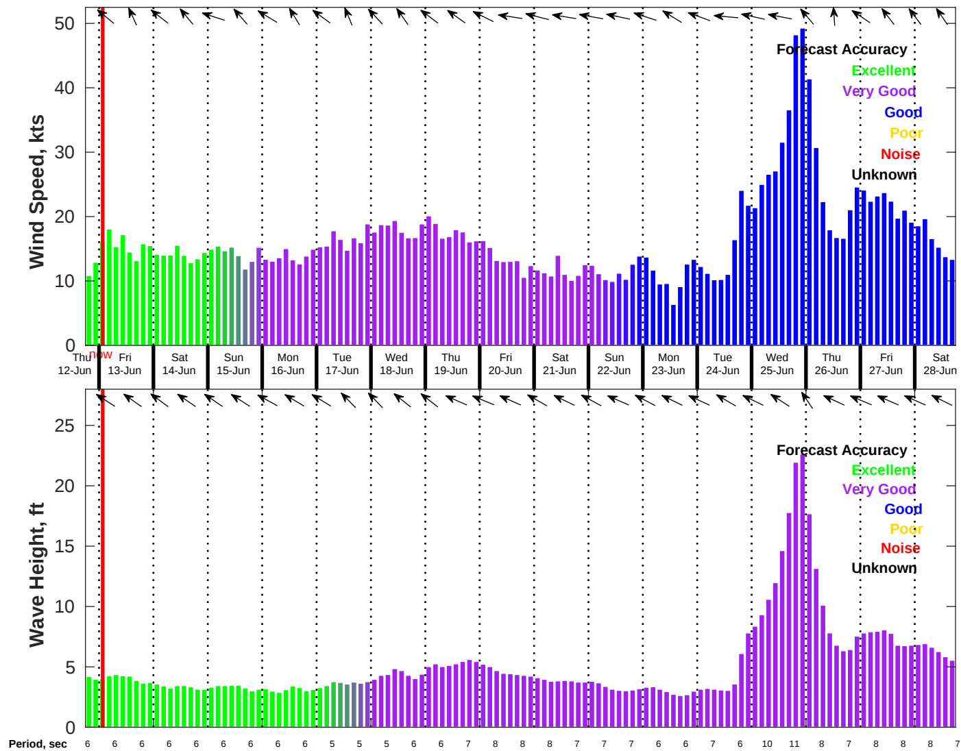
Wind & Wave Forecast for NDBC 42020 from 12-Jun-2025 18:00:00 to 28-Jun-2025 18:00:00
