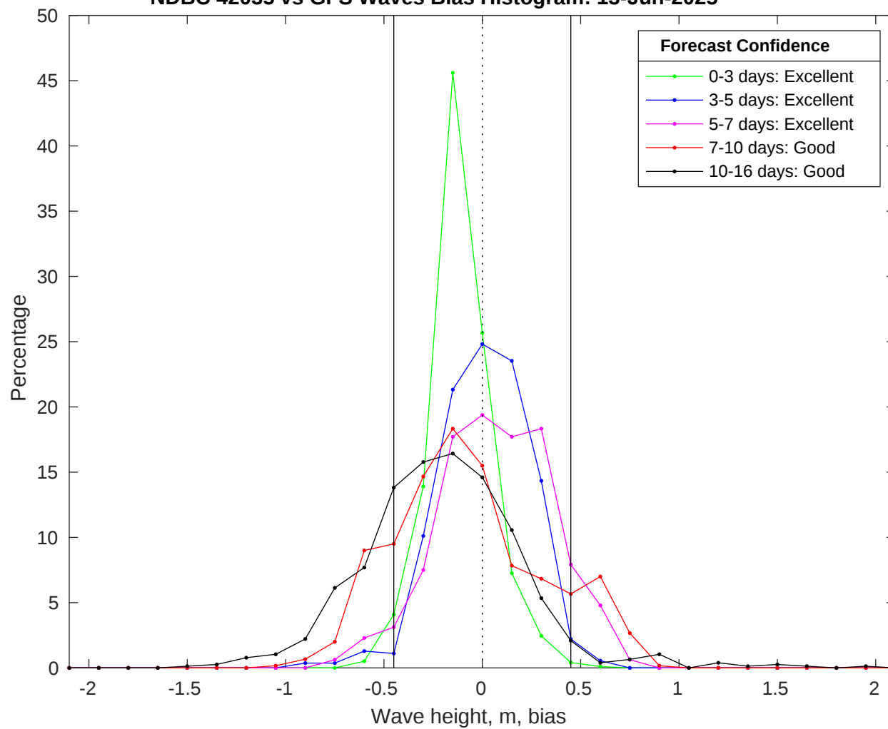
NDBC 42035 vs GFS Waves Bias Histogram: 13-Jun-2025
