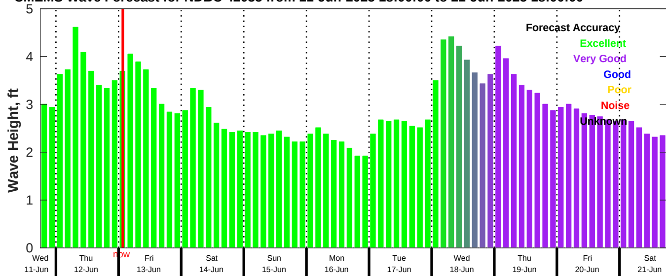
CMEMS Wave Forecast for NDBC 42035 from 11-Jun-2025 18:00:00 to 21-Jun-2025 18:00:00
