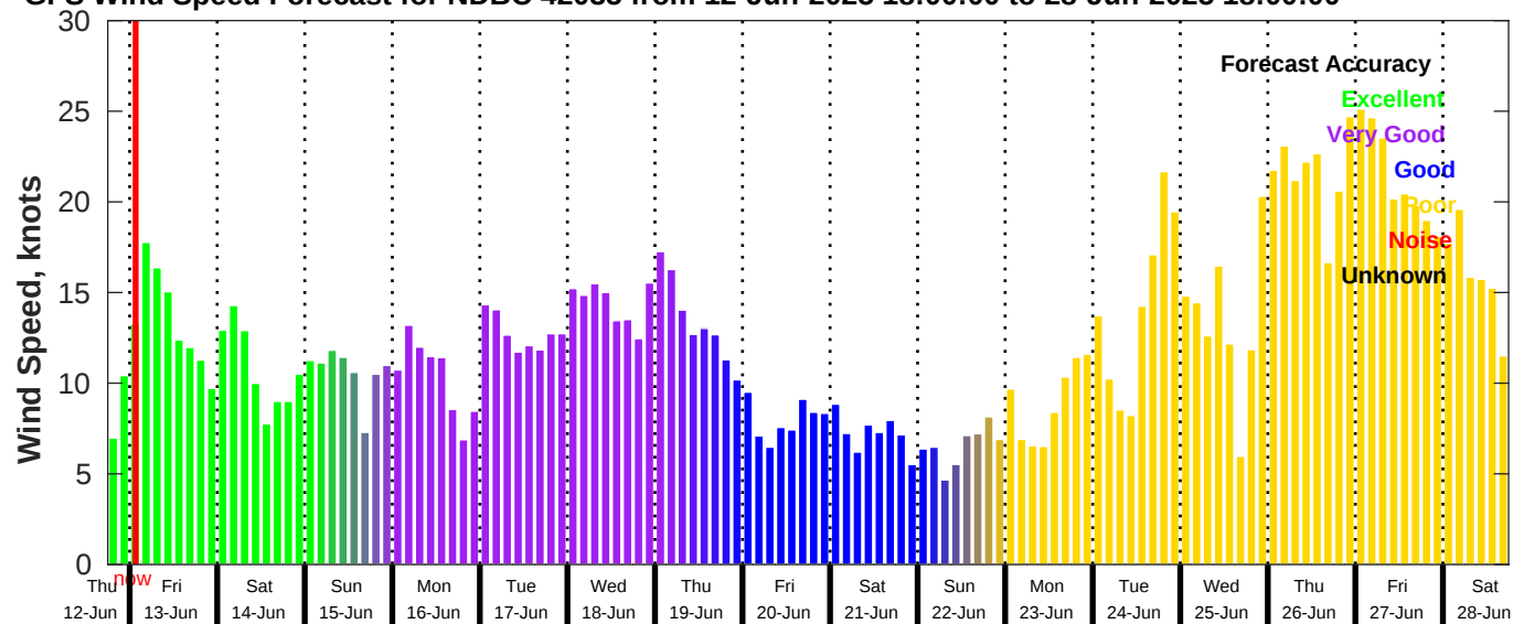
GFS Wind Speed Forecast for NDBC 42035 from 12-Jun-2025 18:00:00 to 28-Jun-2025 18:00:00
