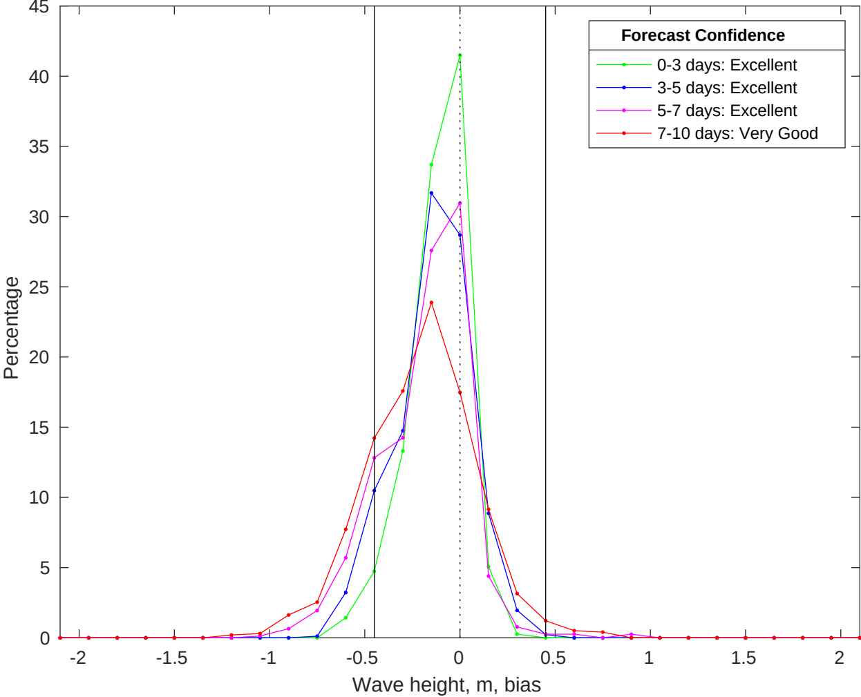
NDBC 42036 vs CMEMS Waves Bias Histogram: 13-Jun-2025
